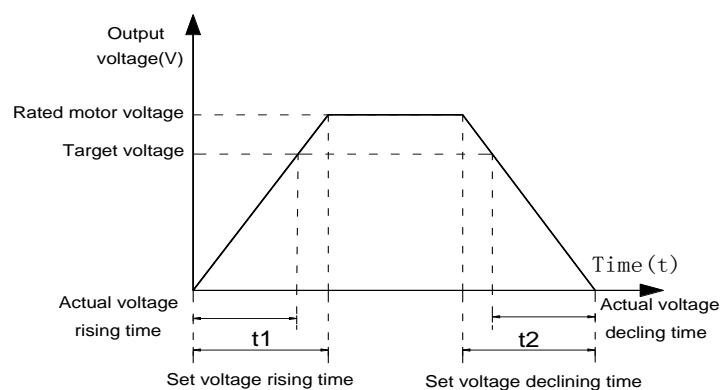
Figure Voltage of V/F separation
